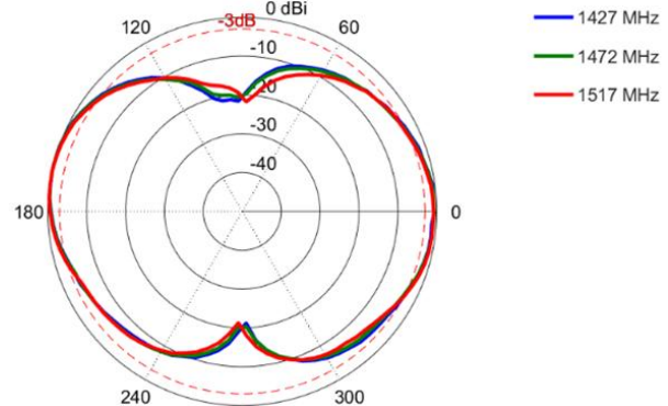
Elevation: 1427 – 1517 MHz
