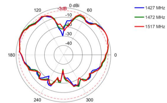
Elevation: 1427 – 1517 MHz
