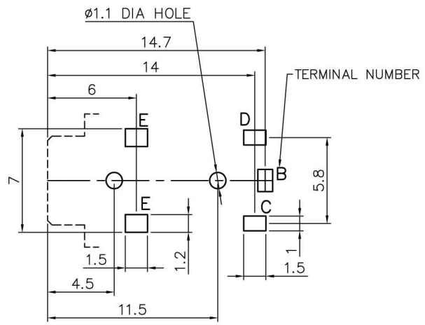
HOLE LAYOUT (BOTTOM VIEW)
